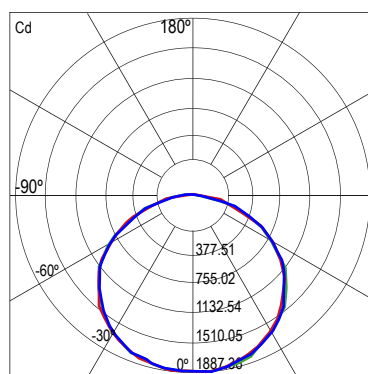
Distribución Polar Candelas / Polar distribution — C0/180 — C90/270 — C157.5 (Max)
