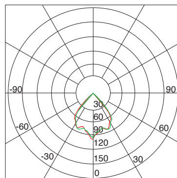
Distribución Polar Candelas Polar distribution Average Beam angle (50%): 81.6 deg.
